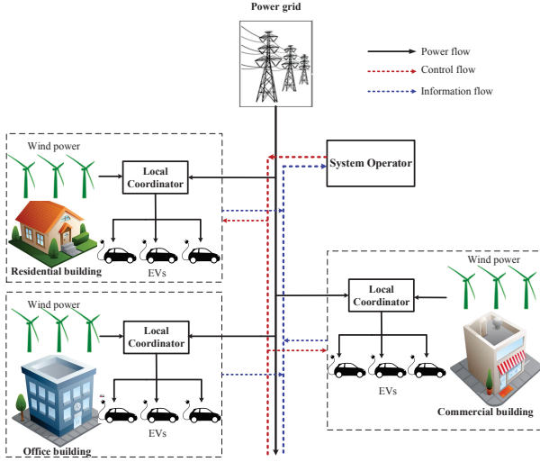
Fig. 2. System Architecture
