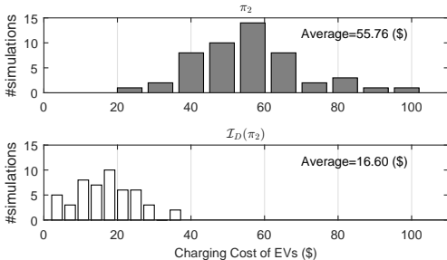
Fig. 6. The distribution of total charging cost of EVs of 50 sample paths with N = 100 EVs using (a) Base policy \pi_2 . (b) Improved policy \mathcal{I}_D(\pi_2) .
