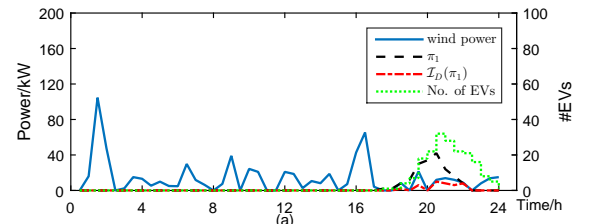
Fig. 9. On-site wind power, the number of EVs, and EV charging power using different policies in commercial building.
