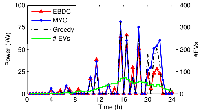
Fig. 9. The amount of power from the power grid at the commercial building ( N = 1000 ).
