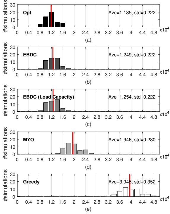
Fig. 7. The unbalance between the EV charging demand of N = 50 EVs and the local wind power supply of the buildings. (a) Optimal. (b) EBDC (without load capacity constraints). (c) EBDC. (d) myopic. (e) Greedy.
