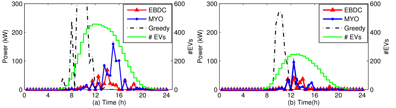
Fig. 11. The amount of power from the power grid at the office buildings ( N = 1000 ). (a) Office I. (b) Office II.
