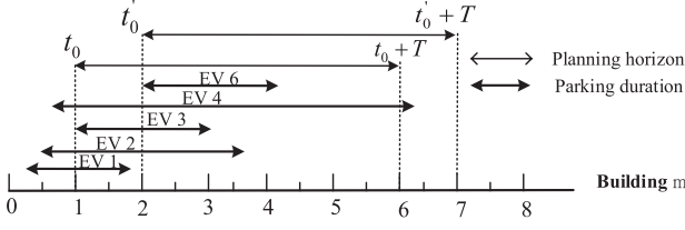
Fig. 3. The current collection of parked vehicles in building m over different planning horizons. \mathcal{N}_m(t_0) = \{1, 2, 3, 4\} , \mathcal{N}_m(t'_0) = \{2, 3, 4, 6\} .
