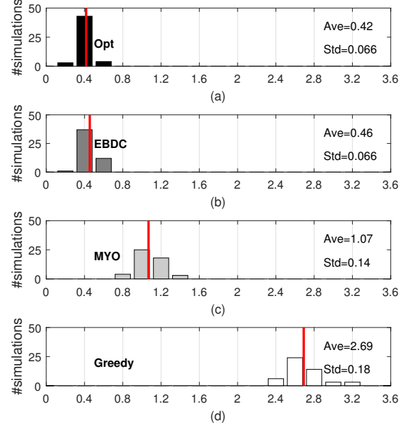
Fig. 13. The unbalance between the EV charging demand of N = 50 EVs and the local renewable energy supply of the buildings. (a) Optimal. (b) EBDC. (c) myopic. (d) Greedy.
