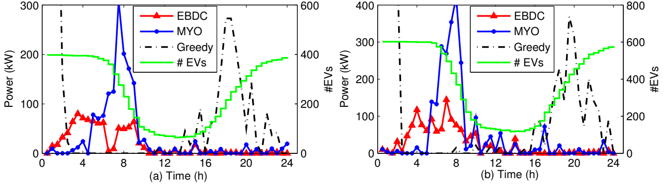
Fig. 10. The amount of power from the power grid at the residential buildings ( N = 1000 ). (a) Residential I. (b) Residential II.
