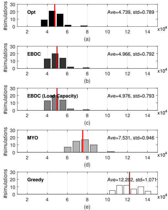
Fig. 8. The unbalance between the EV charging demand of N = 100 EVs and the local wind power supply of the buildings. (a) Optimal. (b) EBDC. (c) EBDC(with load capacity constraints). (d) myopic. (e) Greedy.
